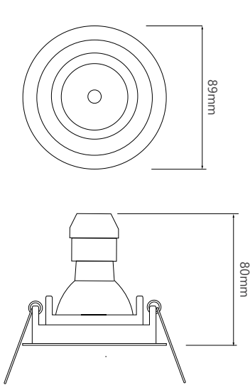
Dimensions using our GU10 LED 5W Retro lamps
