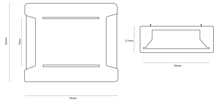
Joiner COB Connectors
