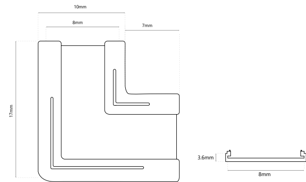
L-ShapedCOBConnectors
