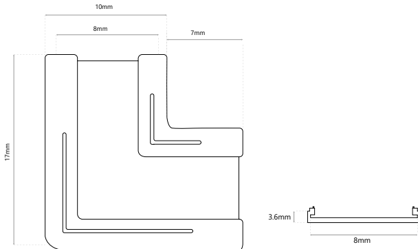
L-Shaped COB Connectors
