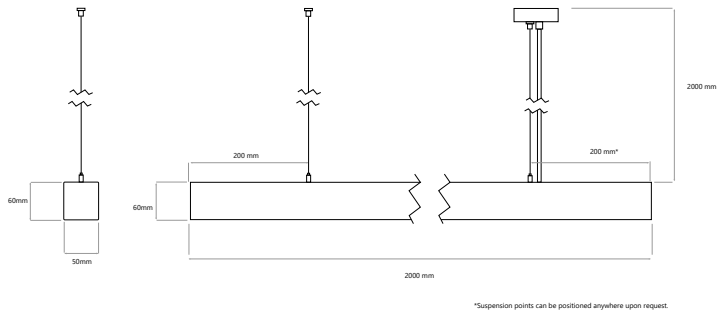
*Suspension points can be positioned anywhere upon request.
