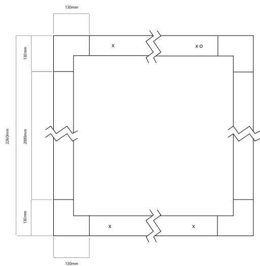
*This drawing represent the basic configuration of 2mx2m profile lenght. Light System Lenght, Suspension Wires and Wire Lenght is completely customizable upon request.
