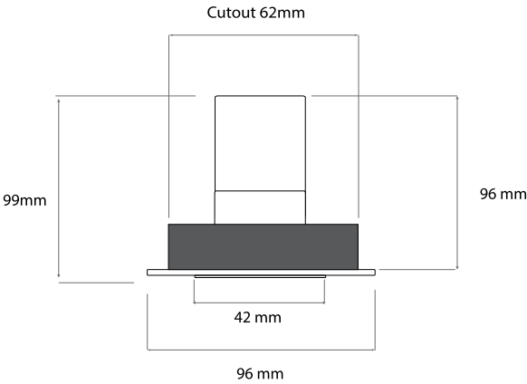
RIGEL 40 Wall-Washer with 9W Module
