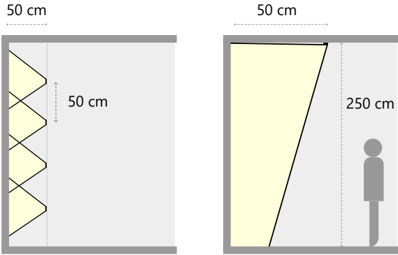
RIGEL TRIMLESS WALL WASHER DOWNLIGHT Installation Recommendation
