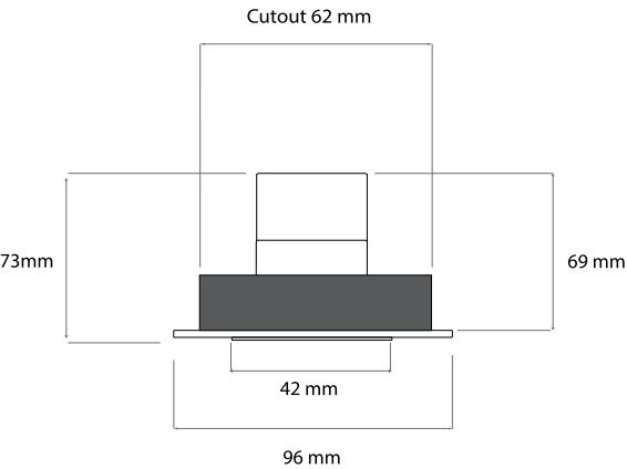
RIGEL 40 Wall-Washer with 7W Module
