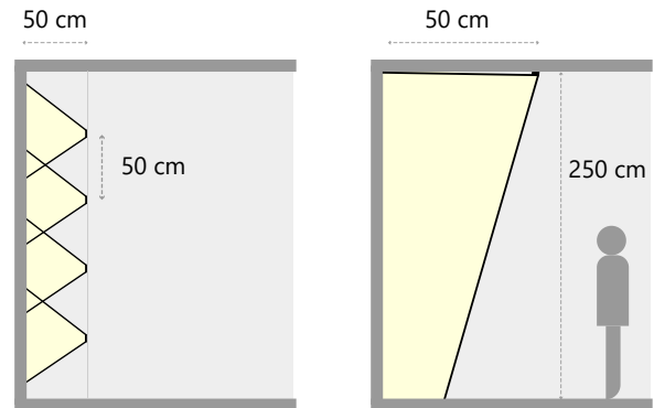
RIGEL TRIMLESS WALL WASHER DOWNLIGHT Installation Recommendation
