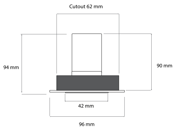
RIGEL 40 Fixed with 9W Module
