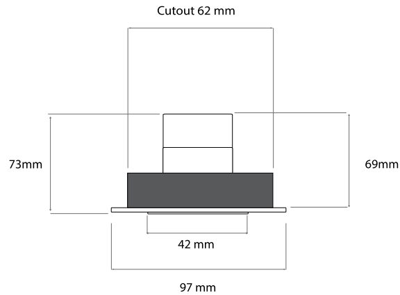
RIGEL 40 Wall-Washer with 7W Module
