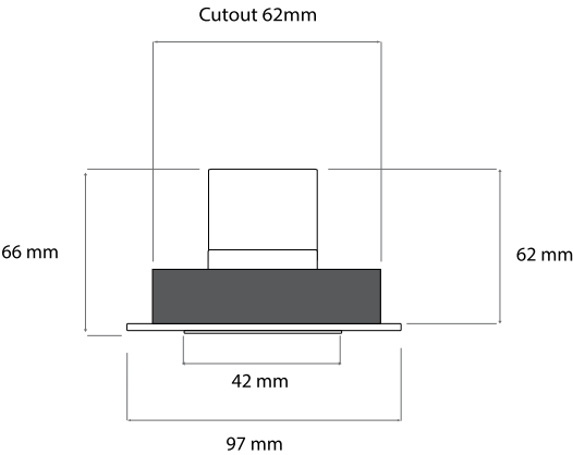
RIGEL 40 Fixed with 7W Module
