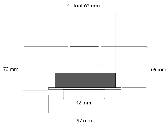
RIGEL 40 Adjustable with 7W Module
