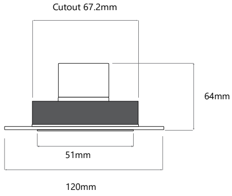
RIGEL 50 with 7WModule
