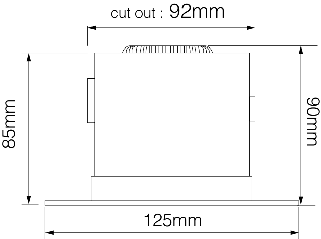
Trimless Downlights with Large GU10 Lamp
