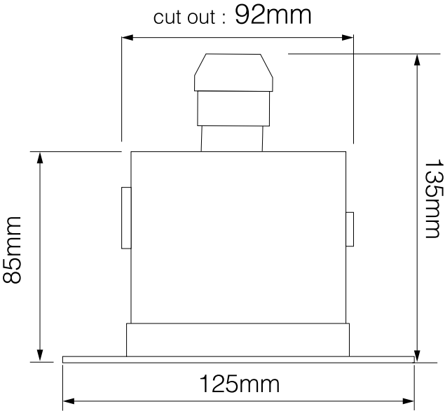
Trimless Downlights with Large GU10 Lamp
