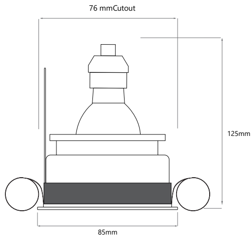
With Baffle
