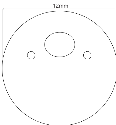
Without End Cap
