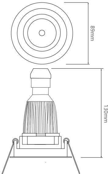
Dimensions using our GU10 LED 7W Large lamps
