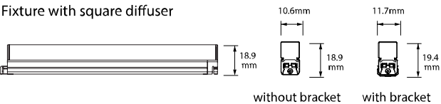
Fixture with square diffuser
