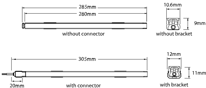
Fixture with flat diffuser
