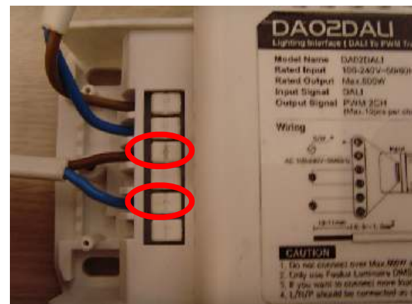
NO.01 DA02DDALI : INPUT SIGNAL DALI
