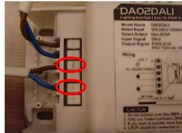
NO.02 DA02DDALI : INPUT SIGNAL DALI
