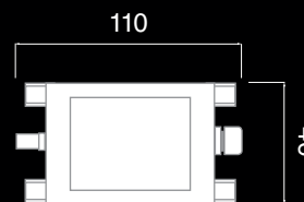
60w Driver
