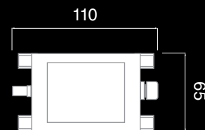
80w Driver
