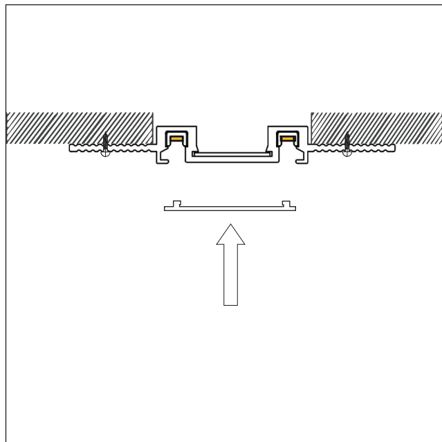
3. Place the protective plastic cover
