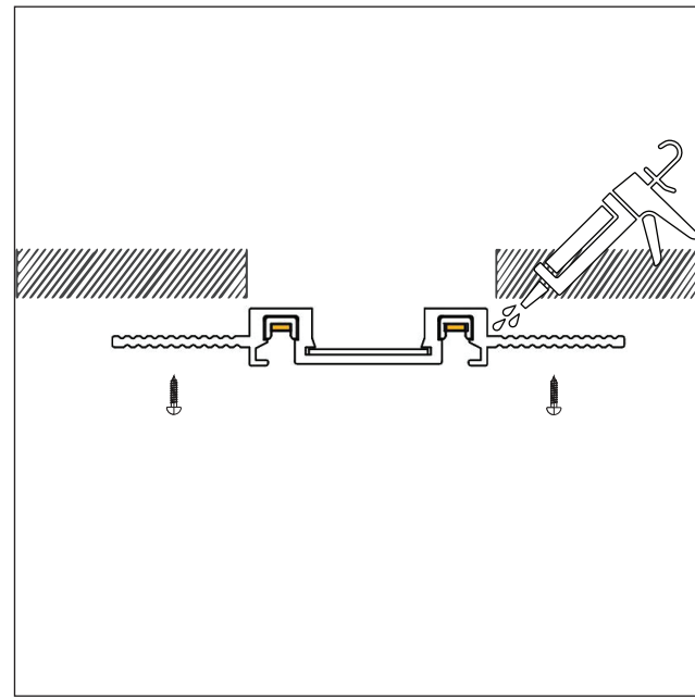
2. Glue and screw the track to the ceiling
