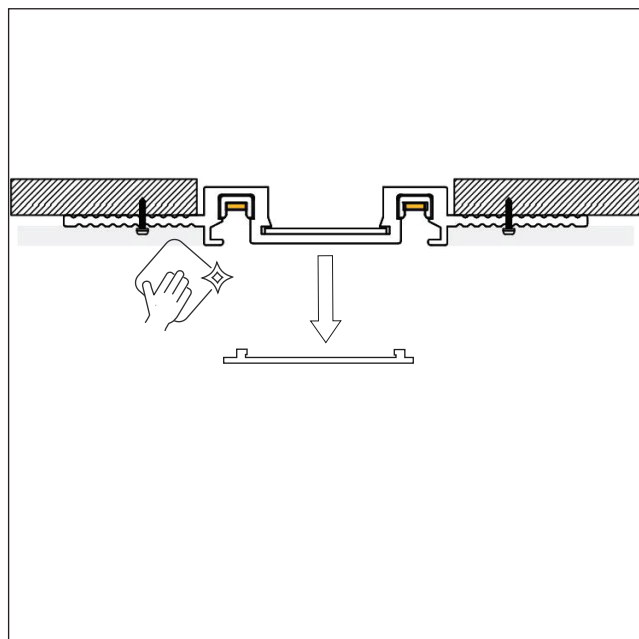
5. Carefully remove the plastic cover and clean the edges.
