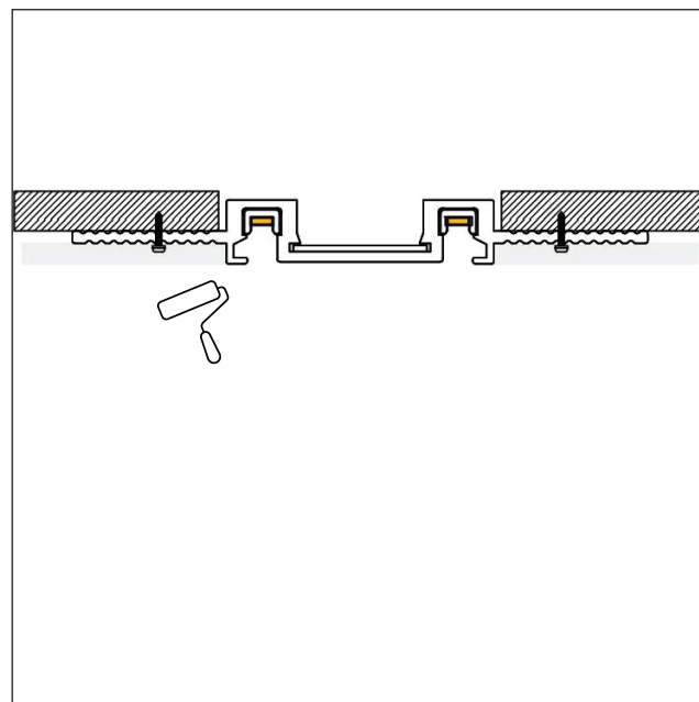
6. Paint the ceiling to achieve a smooth finish
