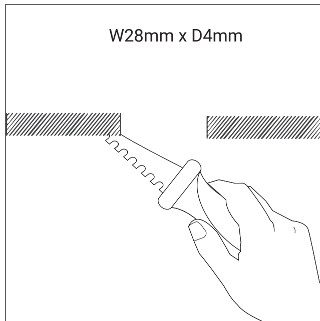
1. Cut hole for the plaster-in track light
